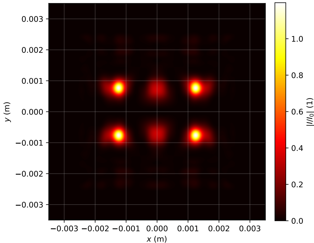
Intensity profile I(x, y, z = 3.105)/I_0 , P_{in}=6.0P_{cr} , artificial time
